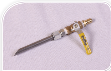
EQ-375BVTI-A Ball Valve Tire Injector Assembly
