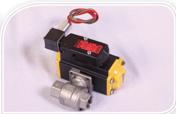
EQ75-SOL-VLV Electronic switched, air- powered Ball Valve
